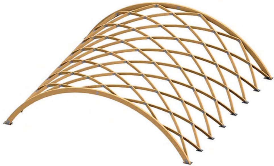
Figure 11. Three-dimensional model of the designed lamella vault.
