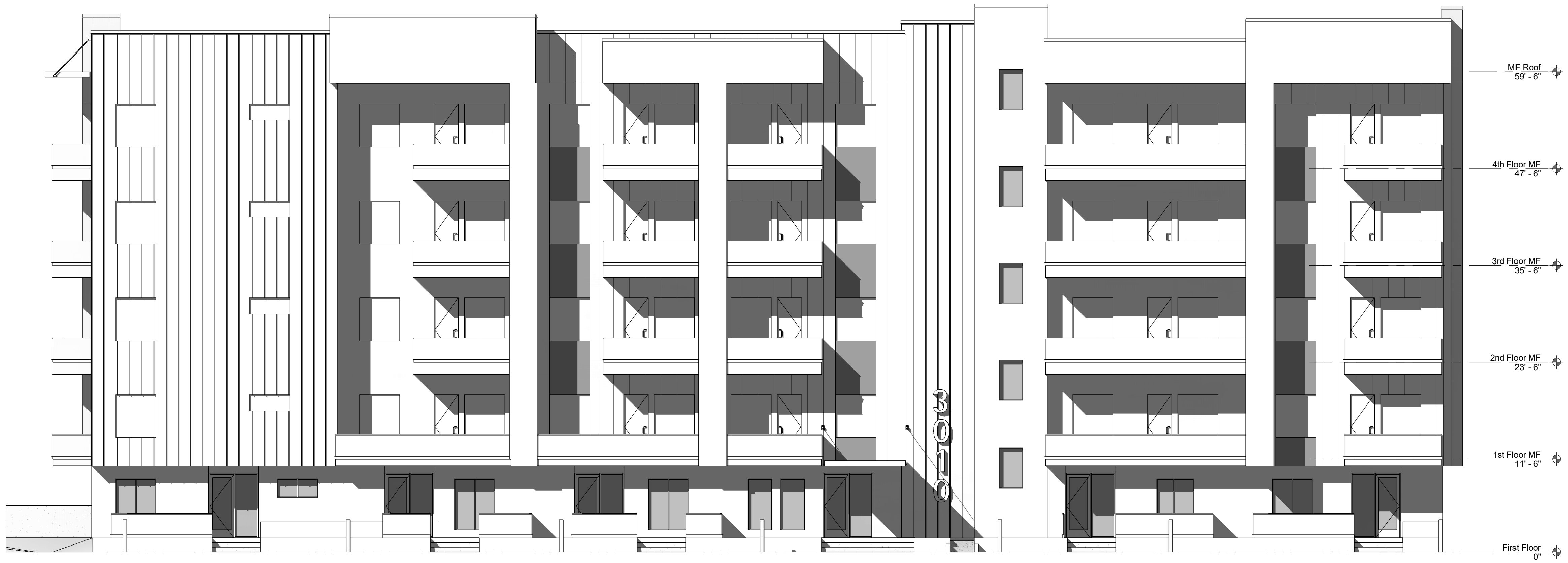
① EAST ELEVATION 1/8" = 1'-0"
