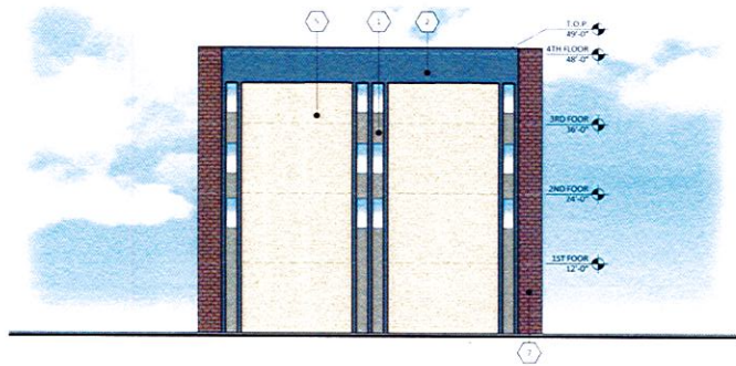
EAST ELEVATION
