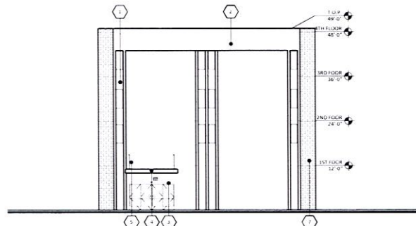
WEST ELEVATION
