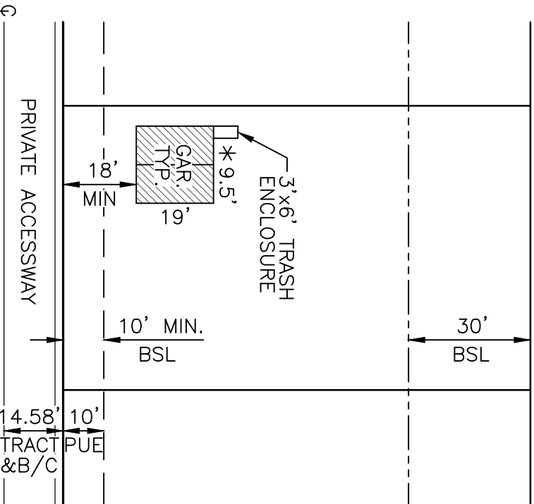
TYPICAL LOT WITHOUT SIDEWALK * MINIMUM 2 SPACES AT 9.5'x19'
