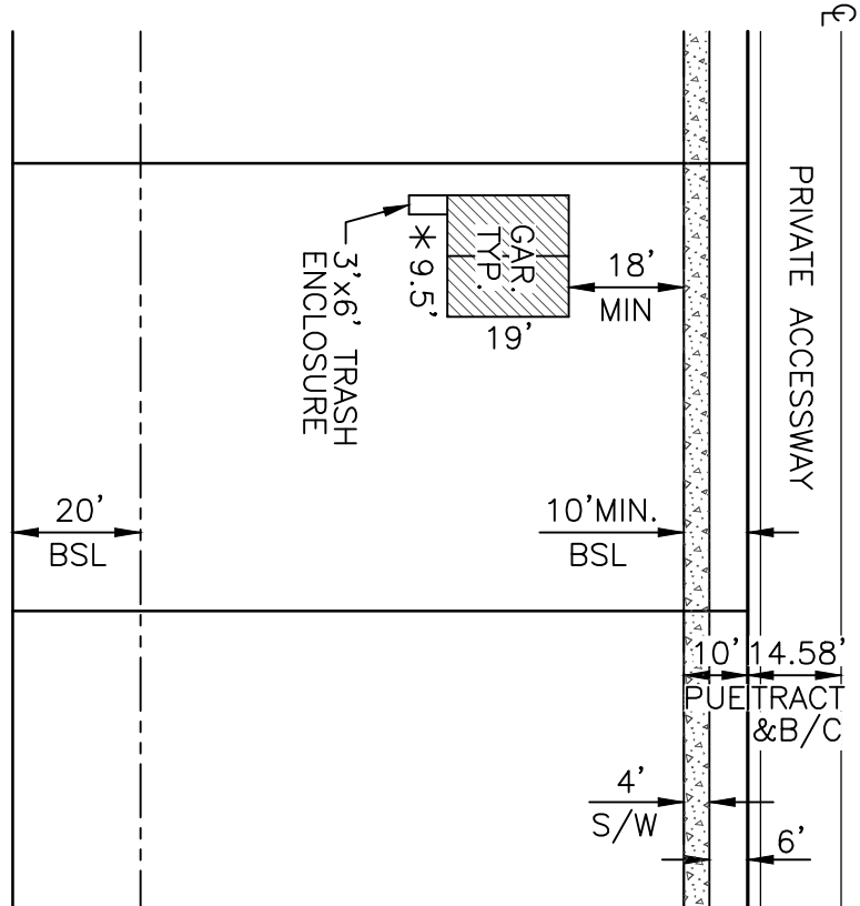
TYPICAL LOT WITH SIDEWALK * MINIMUM 2 SPACES AT 9.5'x19'
