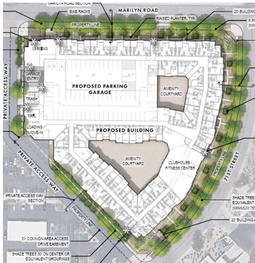
Conceptual Landscape Plan, Source: Collaborative Design Studio
