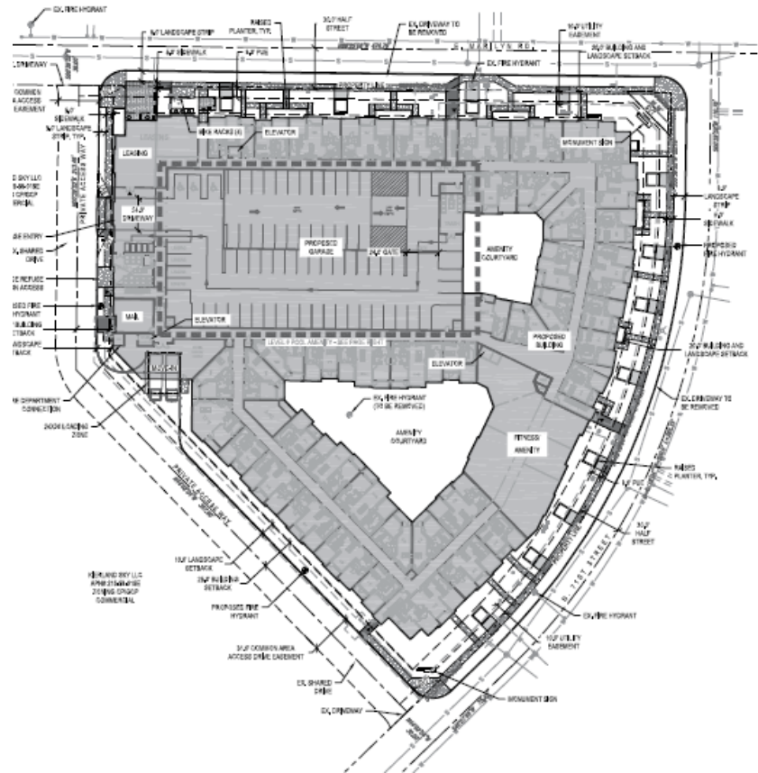
Site Plan, Source: Norris Design
