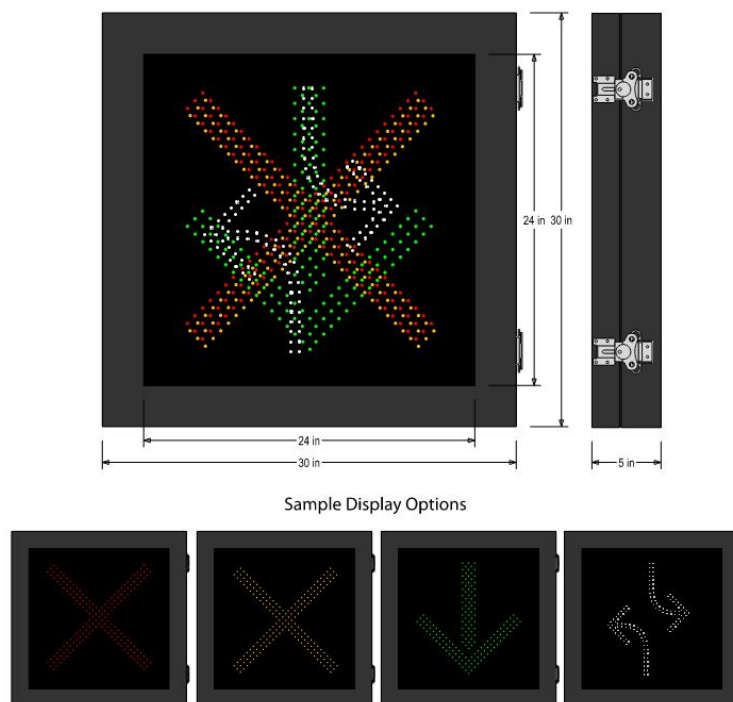
Figure 38 – Sample Mast Arm Dynamic Sign Display
